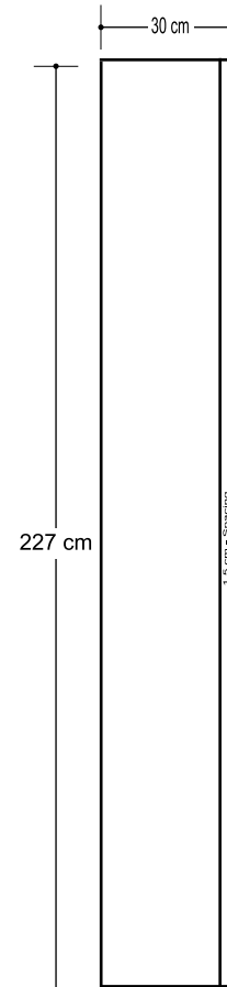
30cm Wing Graphic Panel QTY 2
