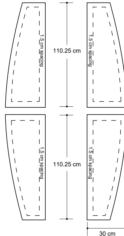
Wings - (4 Pieces)
